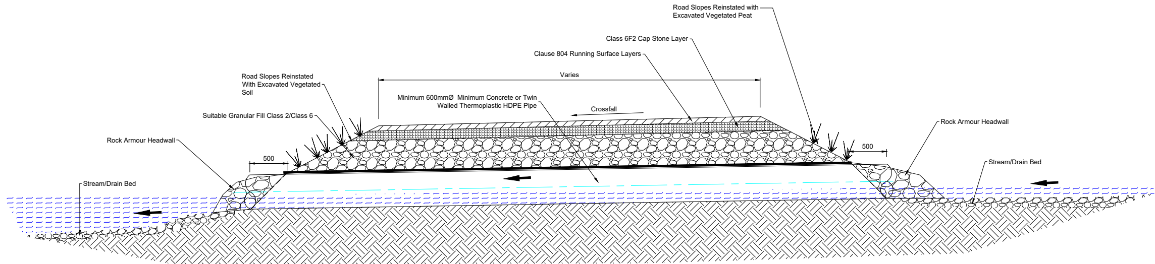
PIPE CULVERT LONG SECTION Scale 1:50
